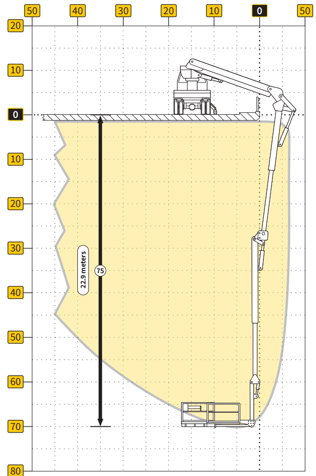
Max Vertical Reach Below Bridge
