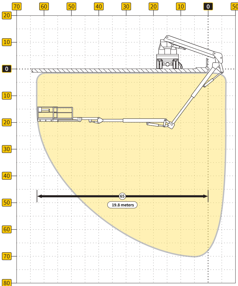
Max Horizontal Reach Under Bridge
